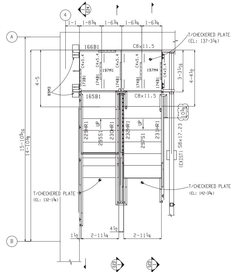
STAIR PLAN AT LEVEL-10 T/STEEL ELEVATION: 137-3 \frac{1}{8} (U.N.)
