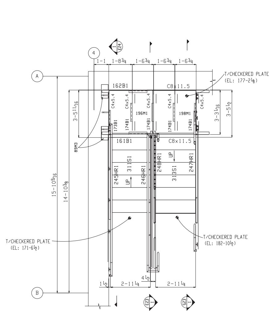
STAIR LANDING PLAN AT EL 177-3 T/STEEL ELEVATION: 177-27 3 / 8 (U.N.)
