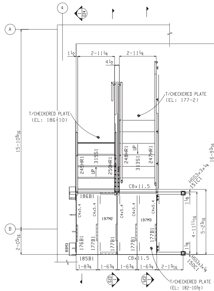
STAIR LANDING PLAN AT EL 182-10 1 / 2 T/STEEL ELEVATION: 182-10 3 / 8 (U.N.)
