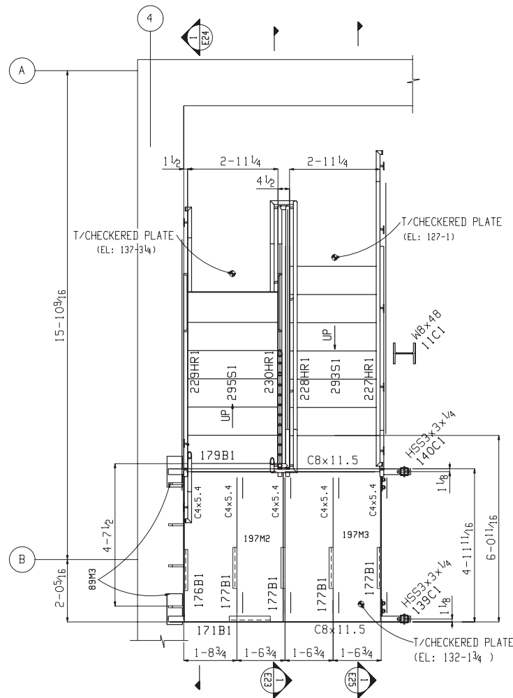
STAIR LANDING PLAN AT EL 132-13 \frac{1}{4} T/STEEL ELEVATION: 132-15 \frac{5}{8} (U.N.)
