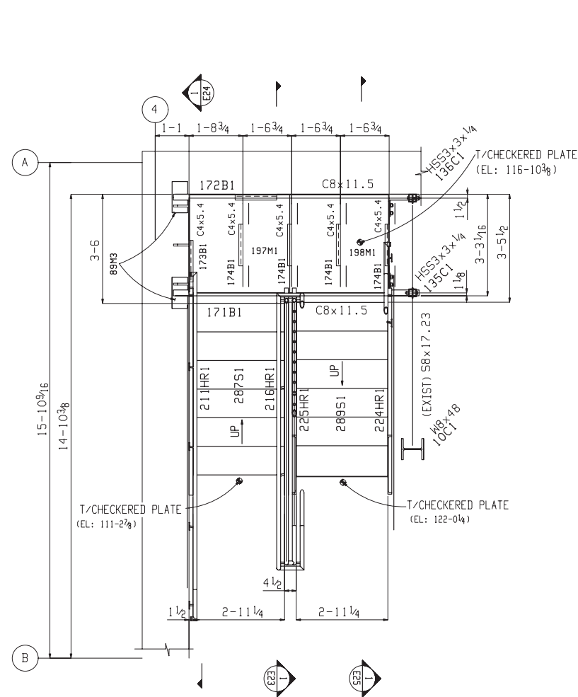
STAIR LANDING PLAN AT EL 116-10 3 / 8 T/STEEL ELEVATION: 116-10 1 / 4 (U.N.)
