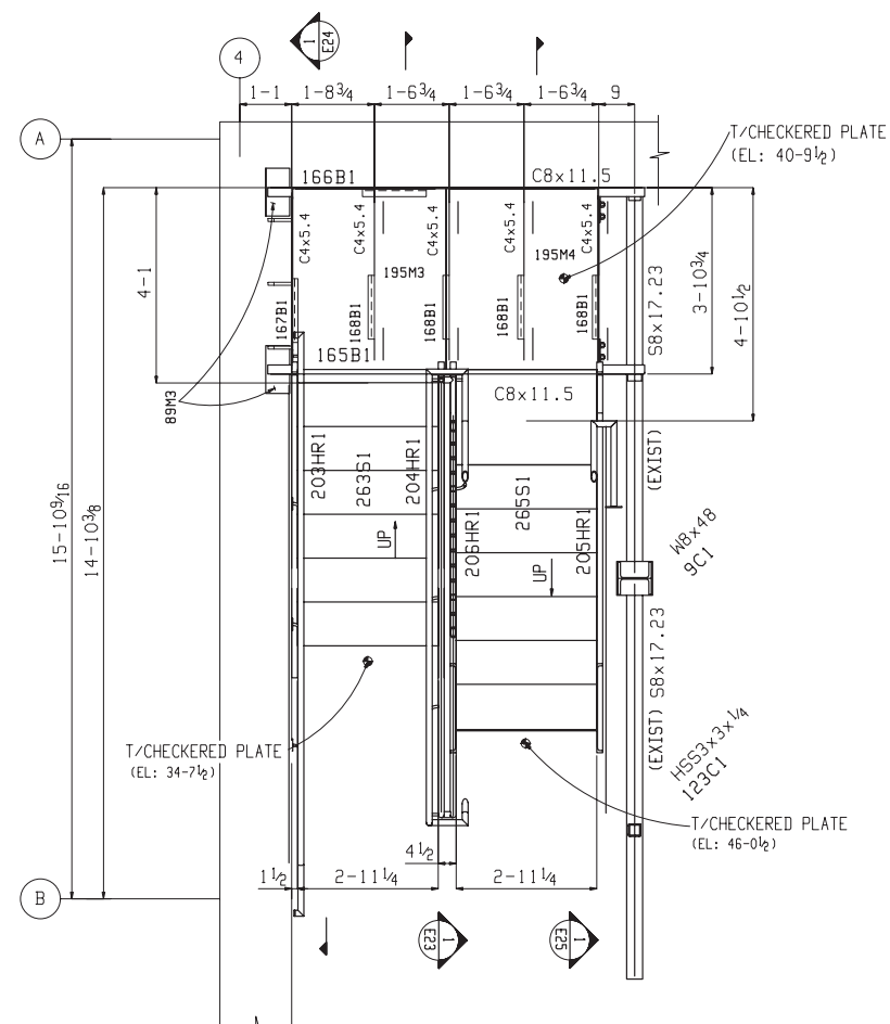
STAIR PLAN AT LEVEL-2 T/STEEL ELEVATION: 40-9 \frac{3}{8} (U.N.) LEVEL-2
