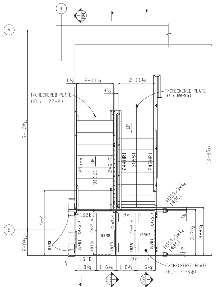
STAIR LANDING PLAN AT EL 171-6 1/2 T/STEEL ELEVATION: 171-6 3/8 (U.N.)
