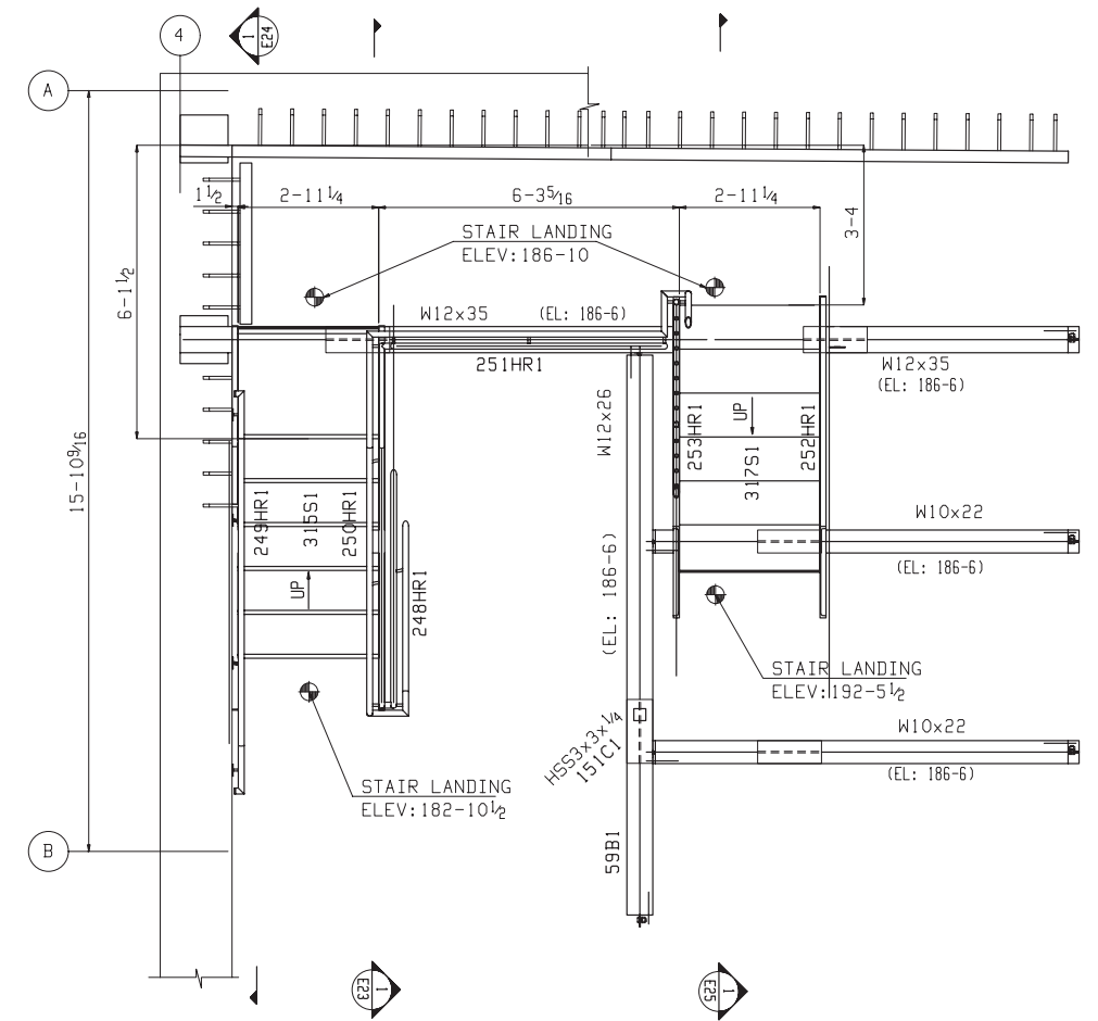
STAIR PLAN AT LEVEL-13 T/STEEL ELEVATION: 186-11 7 / 8 (U.N.)
