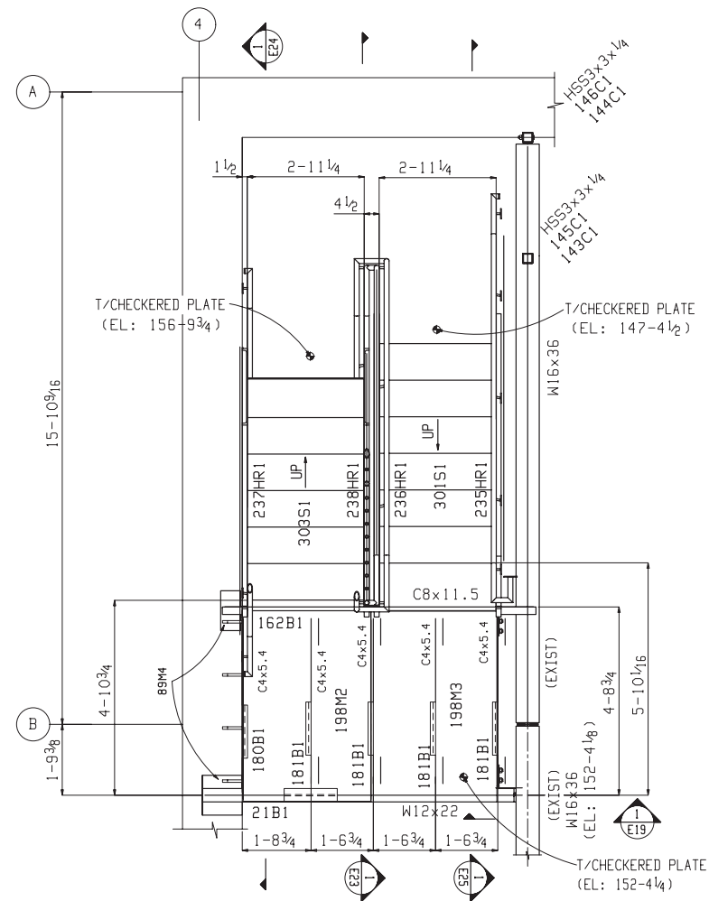
STAIR PLAN AT LEVEL-11 T/STEEL ELEVATION: 152-4 \frac{1}{8} (U.N.)
