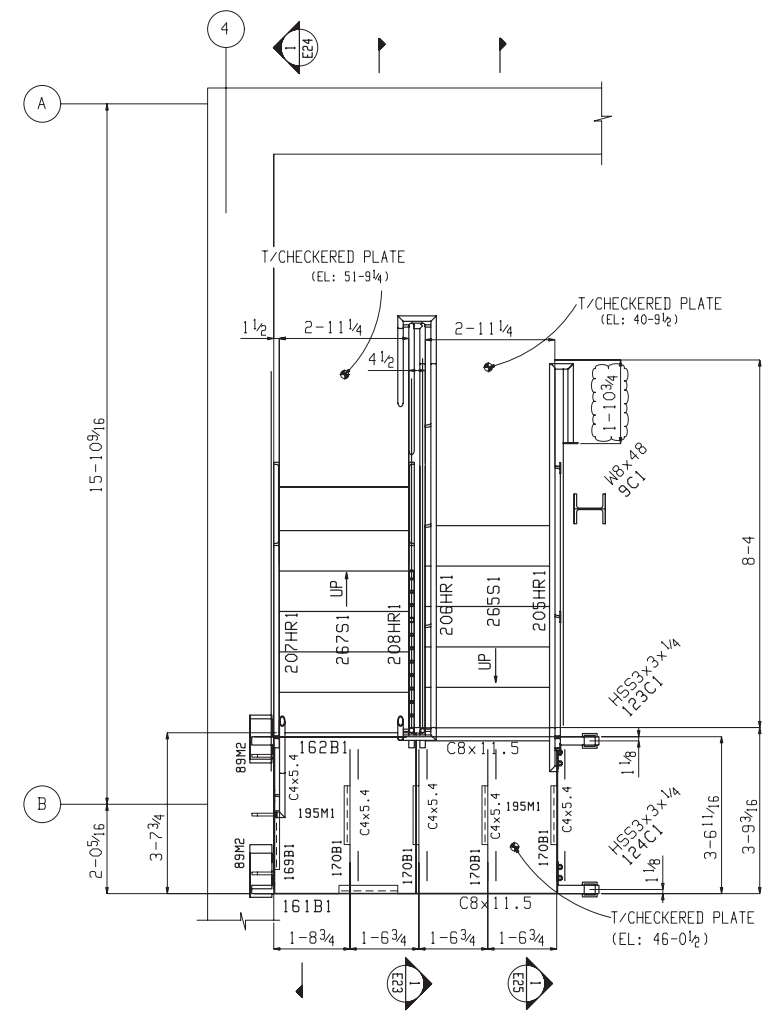
STAIR LANDING PLAN AT EL 46-0 \frac{1}{2} T/STEEL ELEVATION: 46-0 \frac{3}{8} (U.N.)
