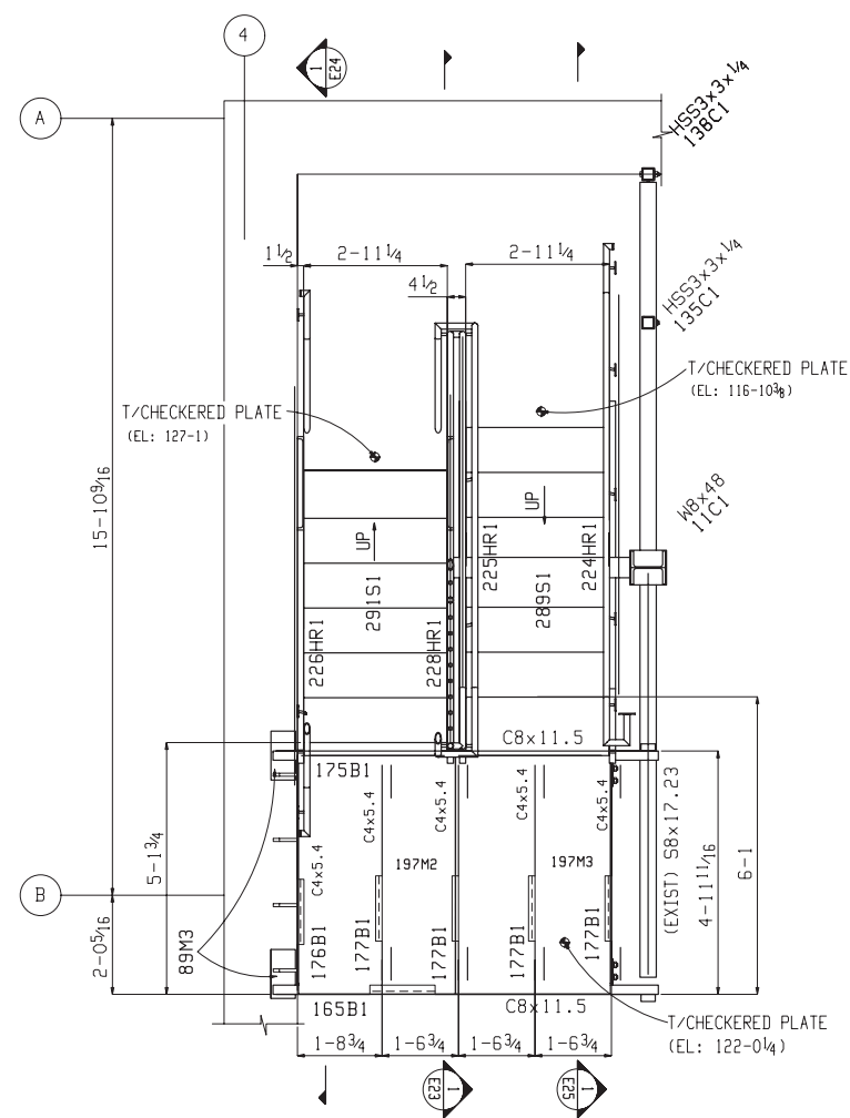
STAIR PLAN AT LEVEL-9 T/STEEL ELEVATION: 122-0 1 / 8 (U.N.)
