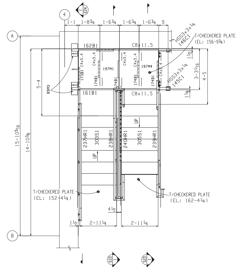
STAIR LANDING PLAN AT EL 156-9 \frac{3}{4} T/STEEL ELEVATION: 156-9 \frac{5}{8} (U.N.)
