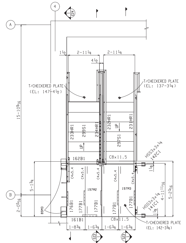
STAIR LANDING PLAN AT EL 142-3 \frac{3}{4} T/STEEL ELEVATION: 142-35 \frac{5}{8} (U.N.)
