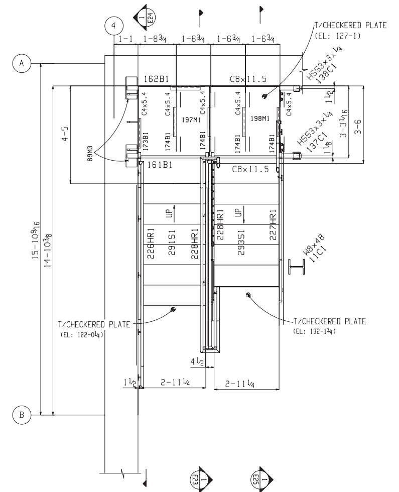
STAIR LANDING PLAN AT EL 127-1 T/STEEL ELEVATION: 127-0 7 / 8 (U.N.)
