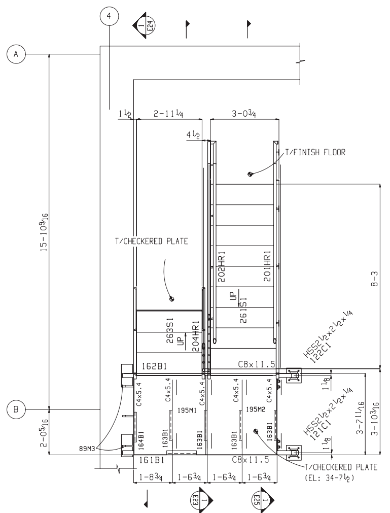
STAIR LANDING PLAN AT EL 34-7 \frac{1}{2} T/STEEL ELEVATION: 34-7 \frac{3}{8} (U.N.)
