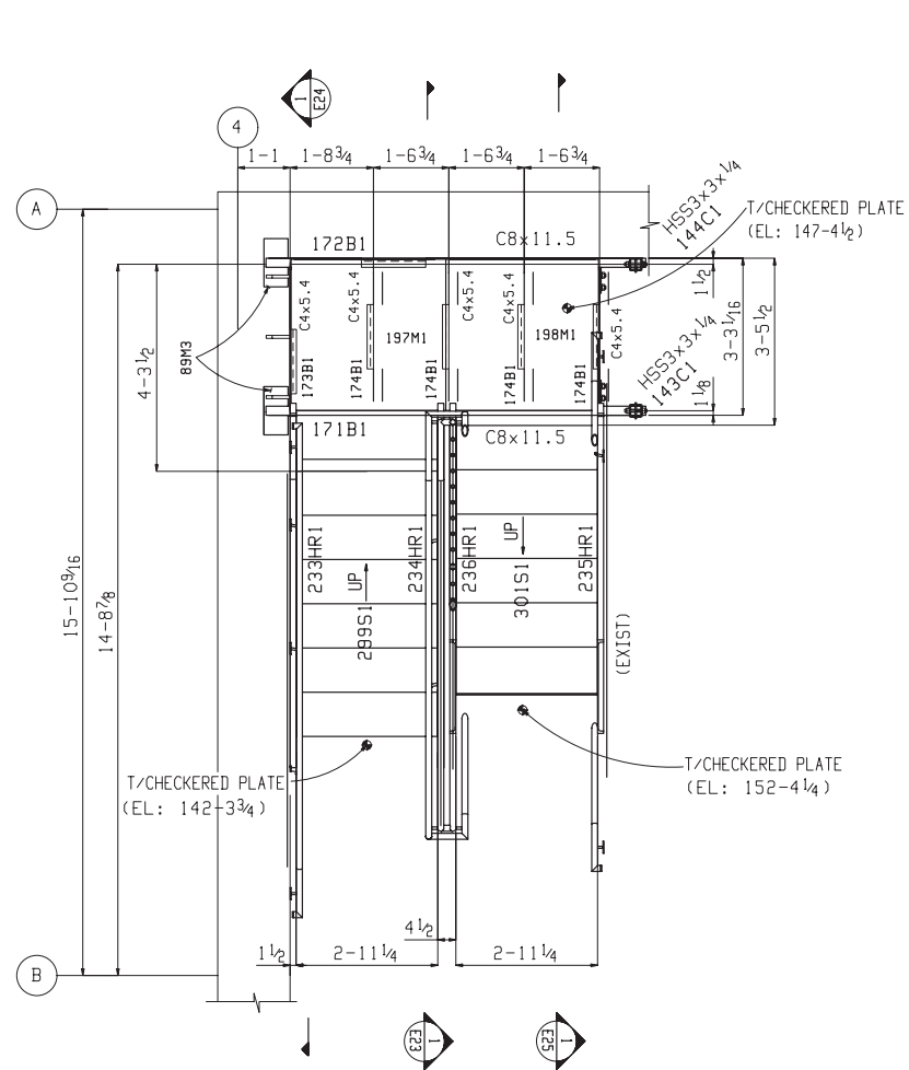
STAIR LANDING PLAN AT EL 147-4 \frac{1}{2} T/STEEL ELEVATION: 147-4 \frac{3}{8} (U.N.)
