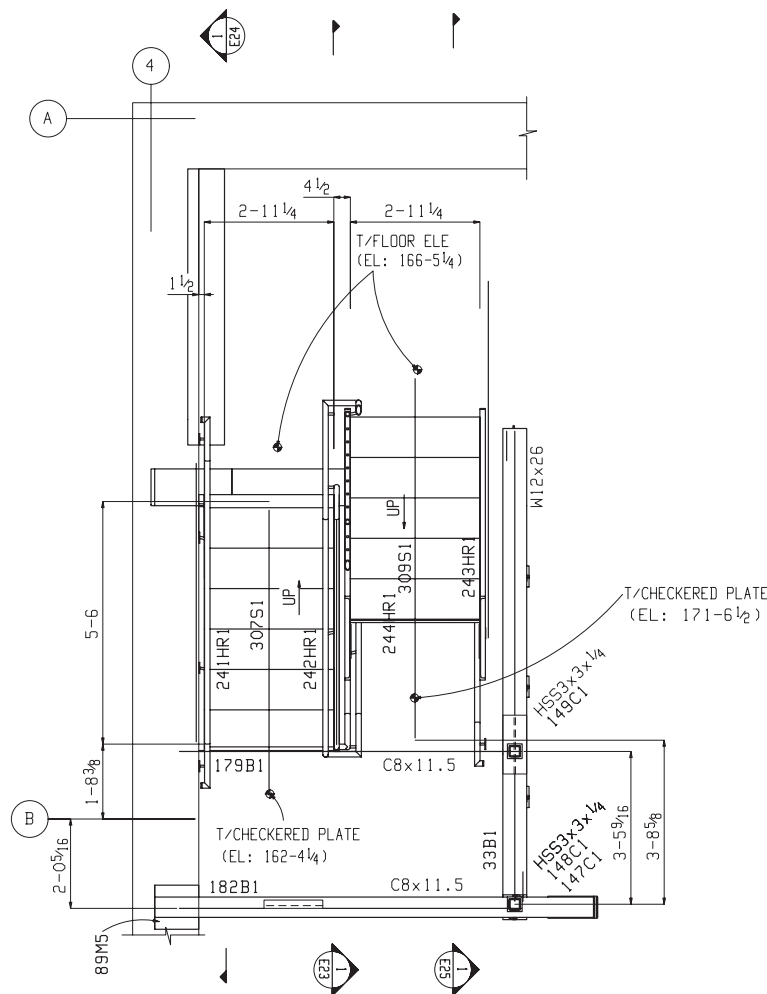
STAIR PLAN AT LEVEL-12 T/STEEL ELEVATION: 166-3 3/8 (U.N.)
