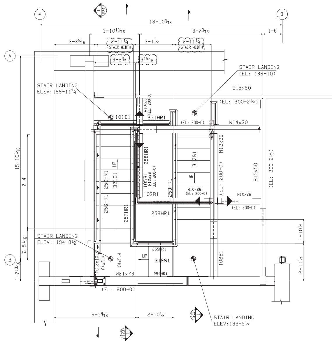
STAIR PLAN AT LEVEL-14 T/STEEL ELEVATION: 199-11 5 / 8 (U.N.)
