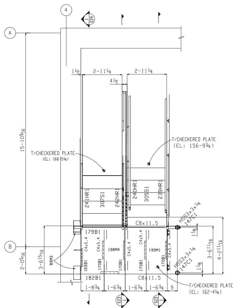
STAIR LANDING PLAN AT EL 162-4 1/4 T/STEEL ELEVATION: 162-4 1/8 (U.N.)
